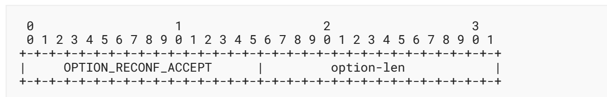
Figure 32: Reconfigure Accept Option Format
