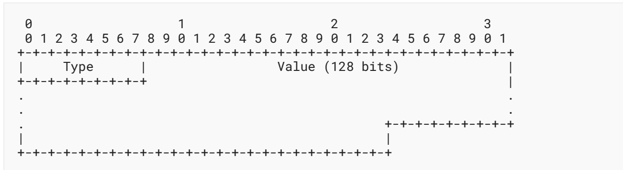
Figure 11: RKAP Authentication Information
