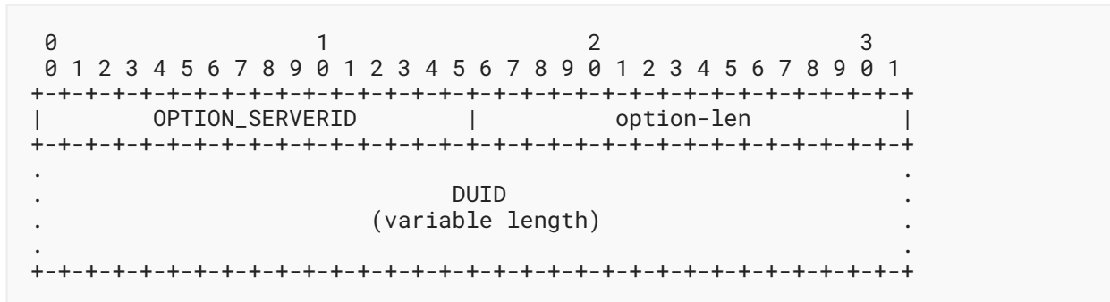
Figure 14: Server Identifier Option Format
