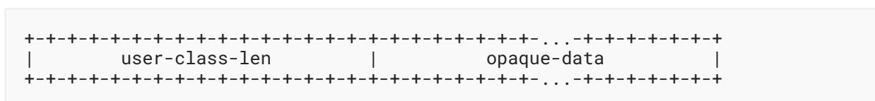
Figure 25: Format of user-class-data Field
