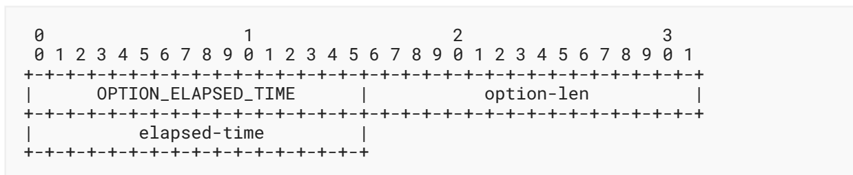
Figure 19: Elapsed Time Option Format
