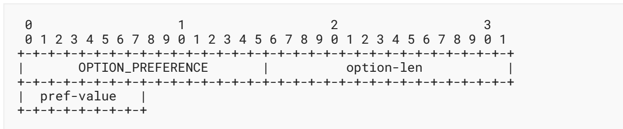
Figure 18: Preference Option Format
